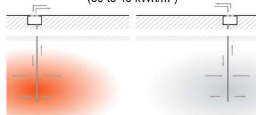
Aquifer thermal energy storage (ATES) (30 to 40 kWh/m 3 )
